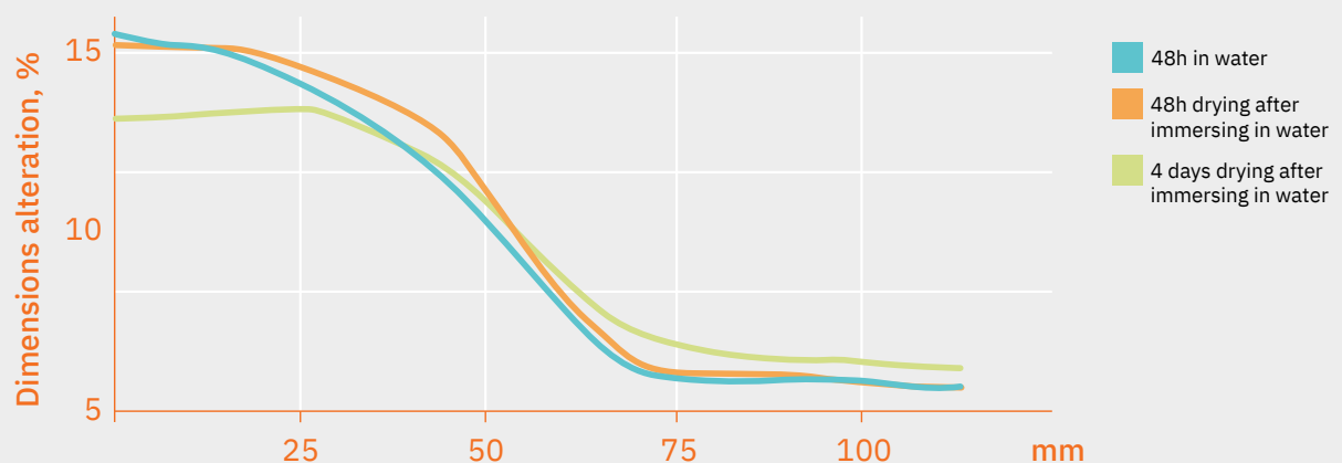
Figure 5.9. Dimension alteration
