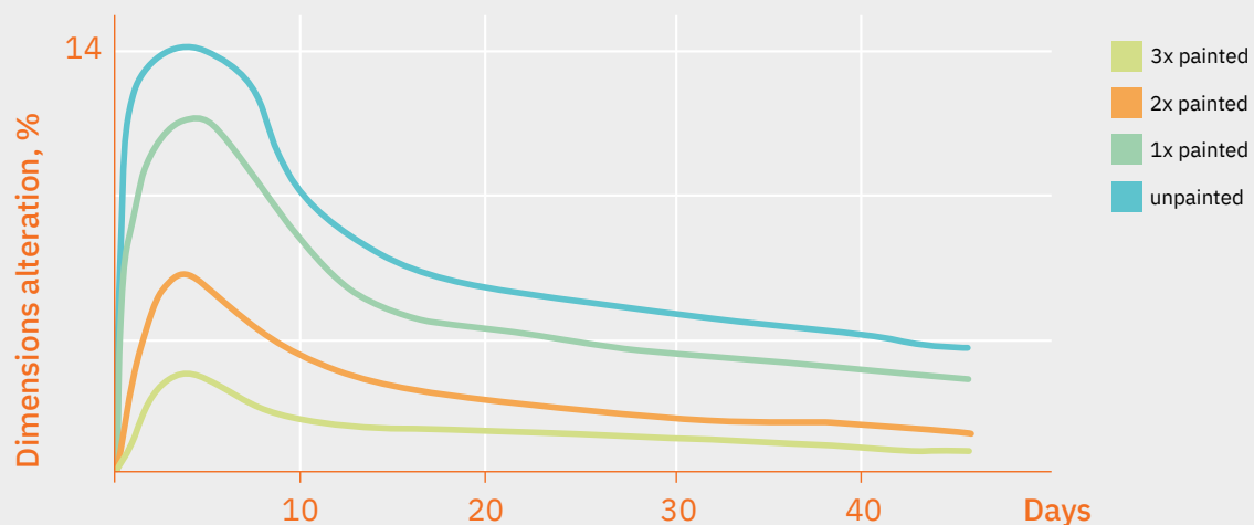
Figure 5.8. Dimension alteration of 18 mm plywood panel overlaid with phenol film, in %, 2 cm from the edge, after immersion in water for 48 h and drying
